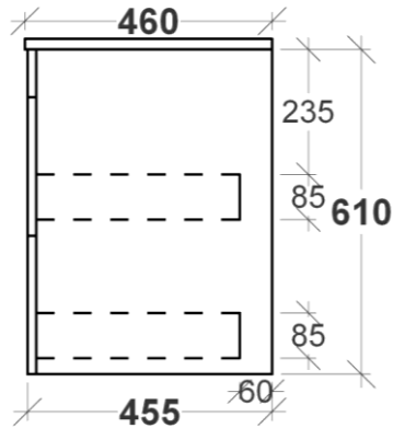
Wall hung side view
