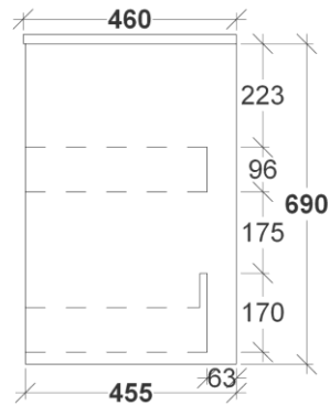
DOUBLE DRAWER FRONT VIEW
