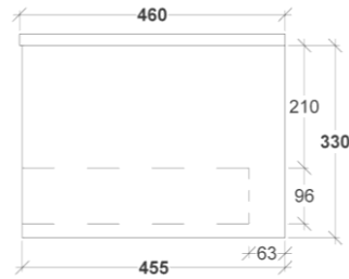
SINGLE DRAWER WALL HUNG SIDE VIEW
