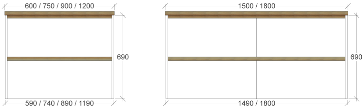
DOUBLE DRAWER FRONT VIEW
