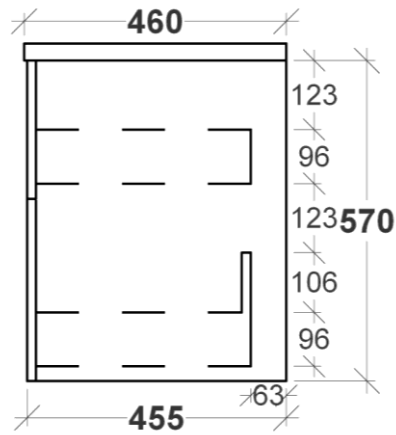
WALL HUNG SIDE VIEW
